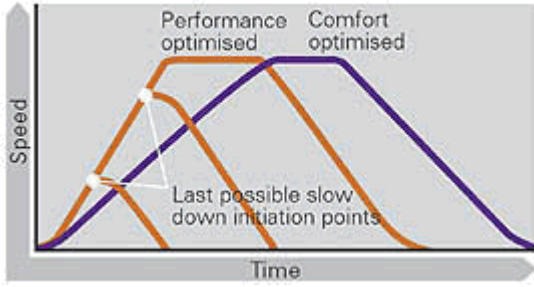
Variodyn performance curve
